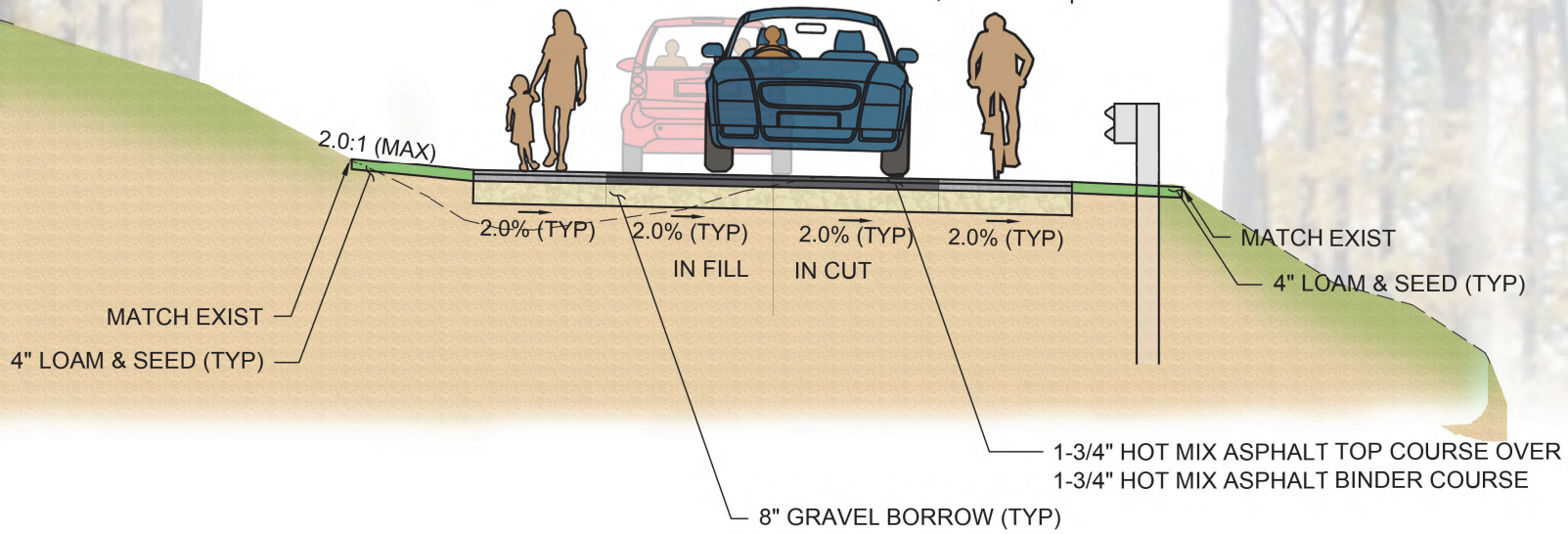
TYPICAL BIKEWAY SECTION
