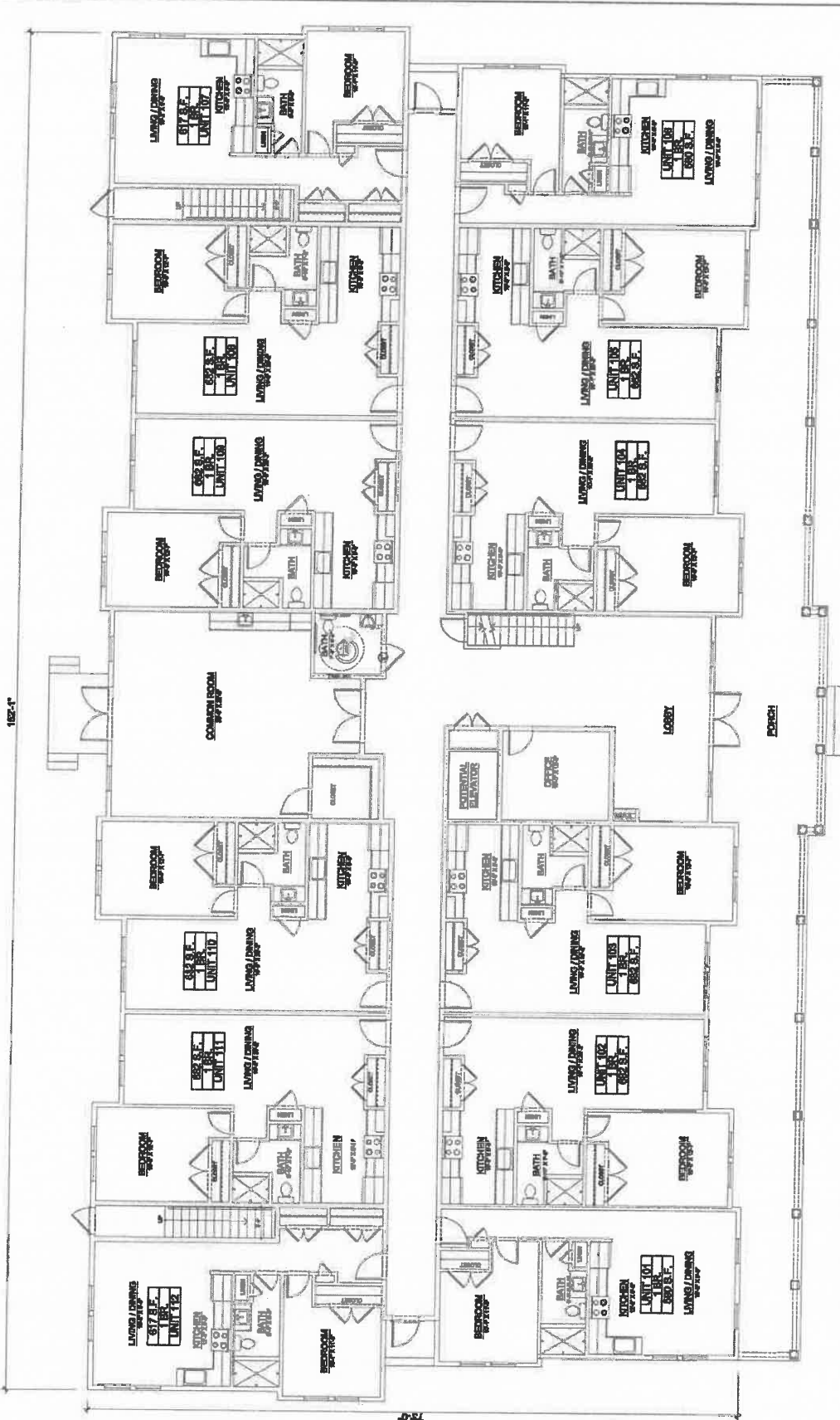
FIRST FLOOR PLAN - SCHEME A
